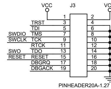
PINHEADER20A-1.27
