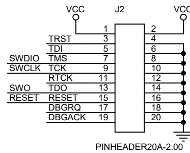
PINHEADER20A-2.00
